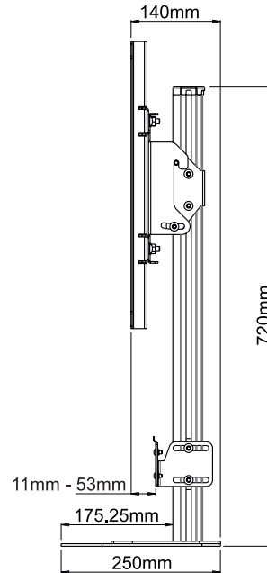
SIDE VIEW (STAND ONLY)
