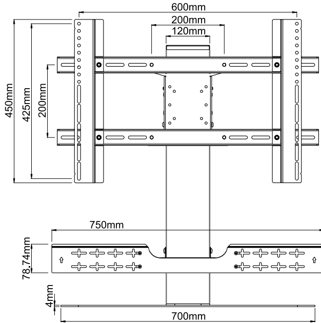
FRONT VIEW (STAND ONLY)
